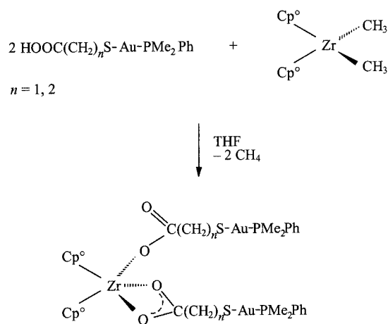
Scheme 1
