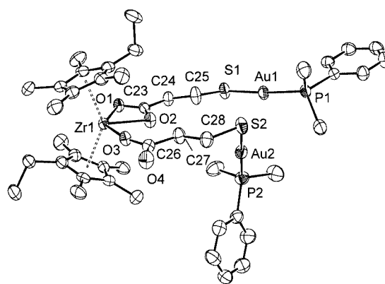
Figure 1. ORTEP plot of 4 (50% probability thermal ellipsoids are shown; hydrogen atoms are omitted for clarity); selected bond lengths [Å] and angles [ ^\circ ]: \text{Zr1}-\text{O1} 2.352(4) , \text{Zr1}-\text{O2} 2.213(4) , \text{Zr1}-\text{O3} 2.067(4) , \text{Au1}-\text{S1} 2.302(2) , \text{Au1}-\text{P1} 2.265(2) , \text{Au2}-\text{S2} 2.306(2) , \text{Au2}-\text{P2} 2.268(2) , \text{O1}-\text{C23} 1.260(7) , \text{O2}-\text{C23} 1.279(6) , \text{O3}-\text{C26} 1.291(7) , \text{O4}-\text{C26} 1.226(7) ; \text{O1}-\text{Zr1}-\text{O2} 56.5(1)^\circ , \text{O2}-\text{Zr1}-\text{O3} 78.9(1)^\circ , \text{S1}-\text{Au1}-\text{P1} 174.63(6)^\circ , \text{S2}-\text{Au2}-\text{P2} 176.83(6)^\circ , \text{O1}-\text{C23}-\text{O2} 117.0(5)^\circ , \text{O3}-\text{C26}-\text{O4} 123.2(6)^\circ
