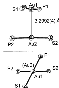
Figure 2. Front and top view of the S–Au–P fragments in 4
